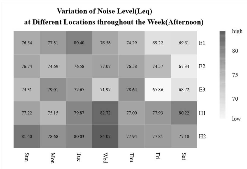
Figure 9: Weekly Variation of L_{eq} (Afternoon)
