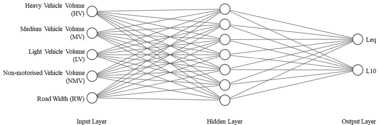
Figure 2: Architecture of neural network model
