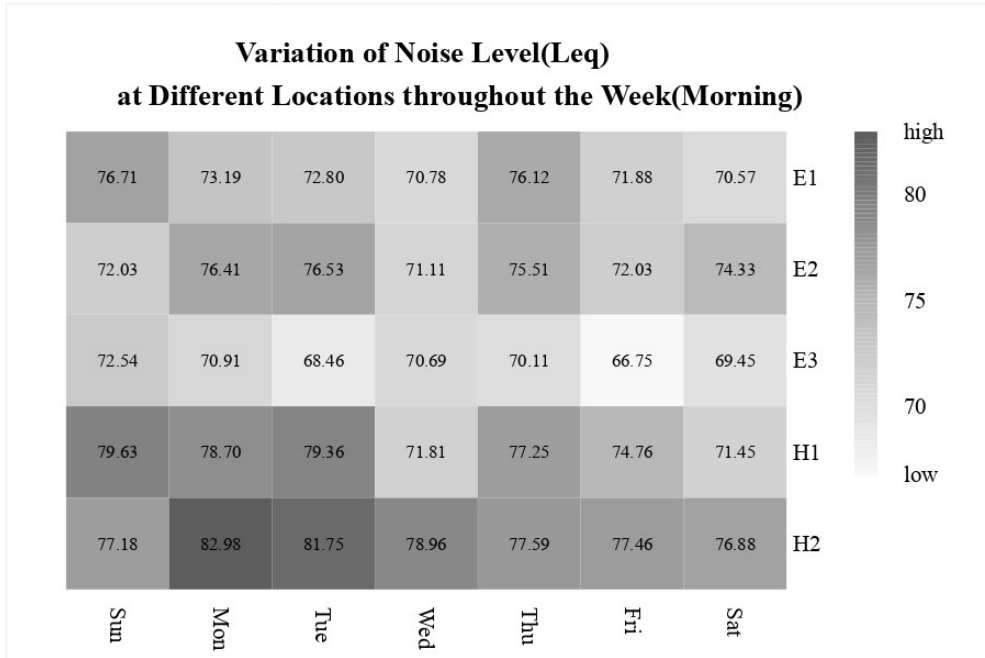
Figure 8: Weekly Variation of L_{eq} (Morning)
