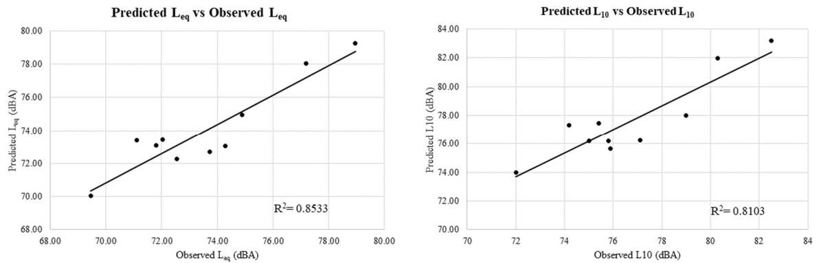
Figure 11: Predicted vs Observed Outputs
