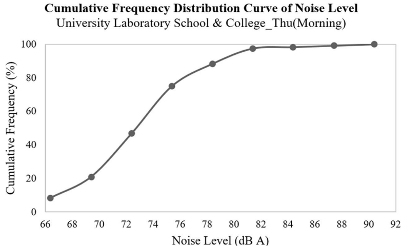
Figure 1: Cumulative Frequency Distribution Curve of Noise Level (E2 Thursday Morning)
