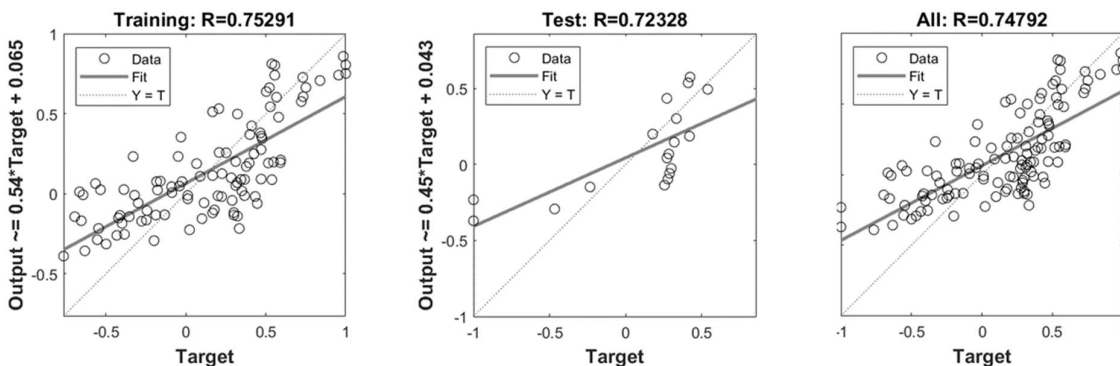
Figure 10: Performance of ANN Model
