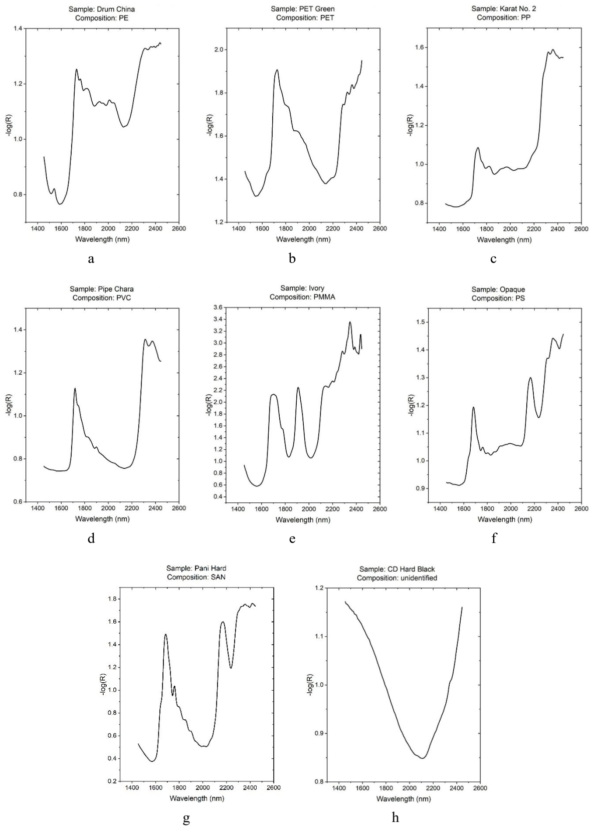
Figure 5. Graphs Obtained from NIR Spectroscopy: a. Graph of PE Plastic, b. Graph of PET Plastic, c. Graph of PP Plastic, d. Graph of PVC Plastic, e. Graph of PMMA Plastic, f. Graph of PS Plastic, g. Graph of SAN Plastic, h. Graph of Unidentified Materials
